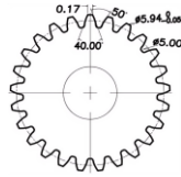
6mm25T Output Shaft Spline
