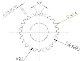
25T 5mm Output Shaft Spline
