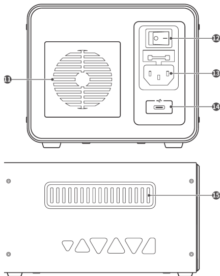
Rear panel and side wall
